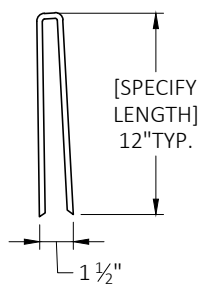
STAPLE TYPE 2
