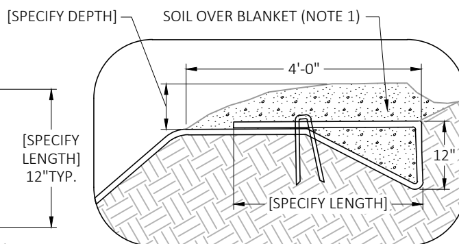
STAPLE ENLARGEMENT
